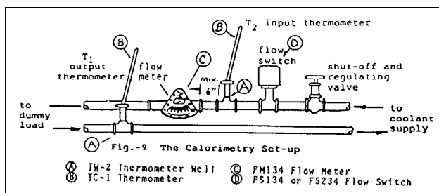
Fig. 9 The Calorimetry Set-up
